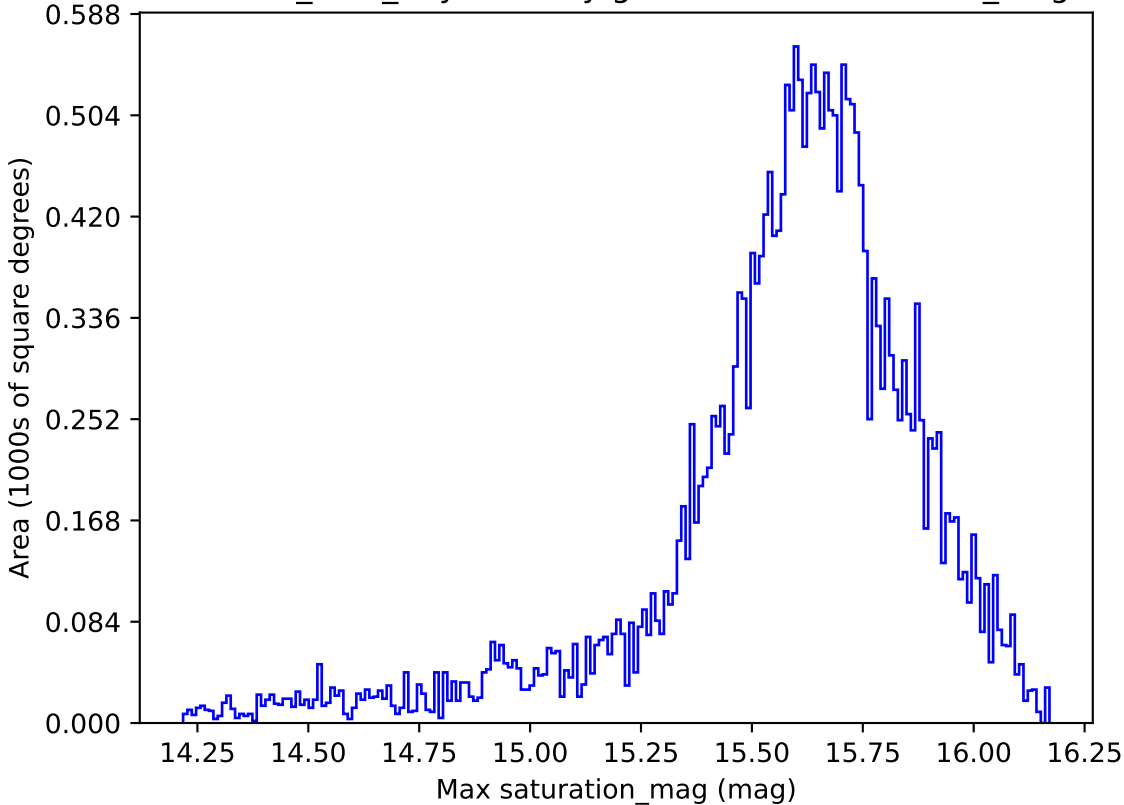
baseline_v3.0_10yrs All sky g band: Max saturation_mag
