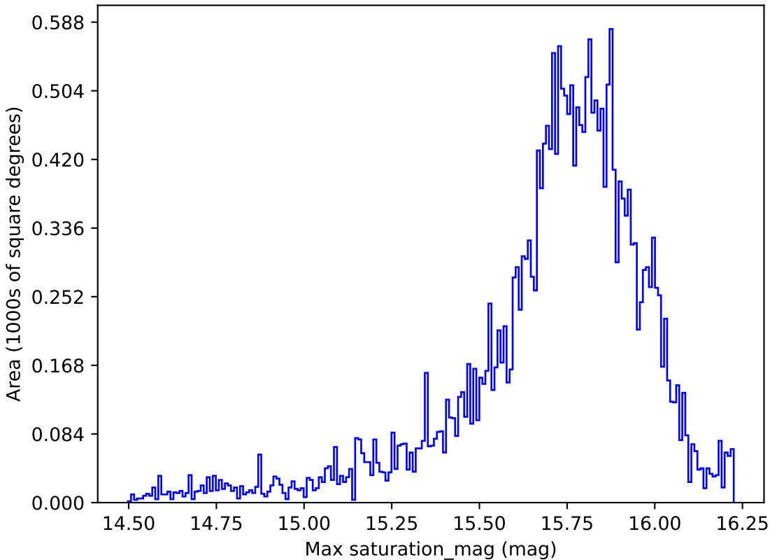
baseline_v3.0_10yrs All sky all bands: Max saturation_mag
