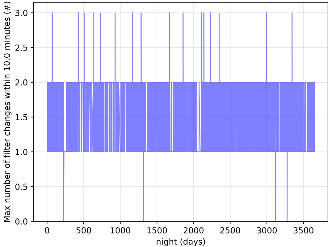
baseline_v3.0_10yrs Per Night: Max number of filter changes within 10.0 minutes
