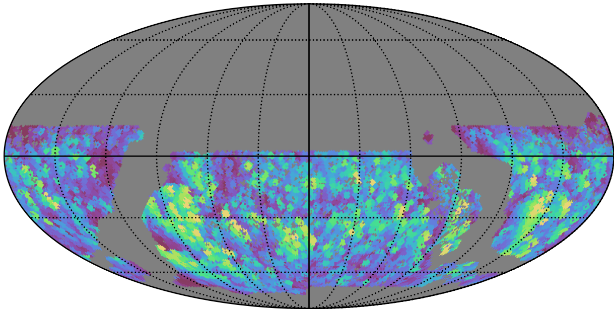
baseline_v3.0_10yrs WFD z band: Max normairmass
