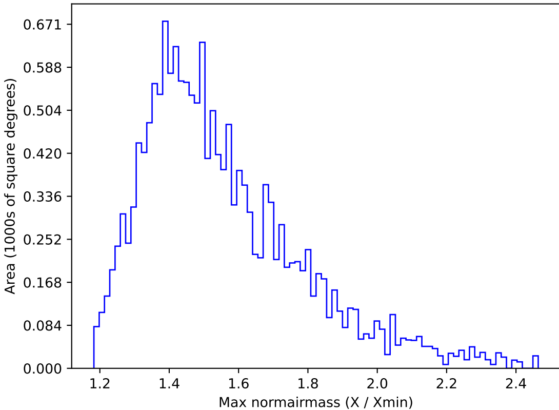
baseline_v3.0_10yrs WFD u band: Max normairmass
