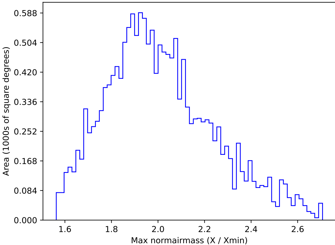
baseline_v3.0_10yrs WFD r band: Max normairmass
