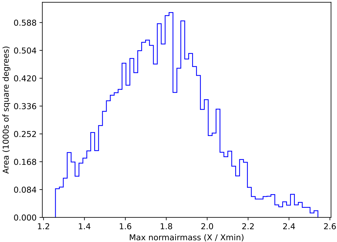
baseline_v3.0_10yrs WFD g band: Max normairmass
