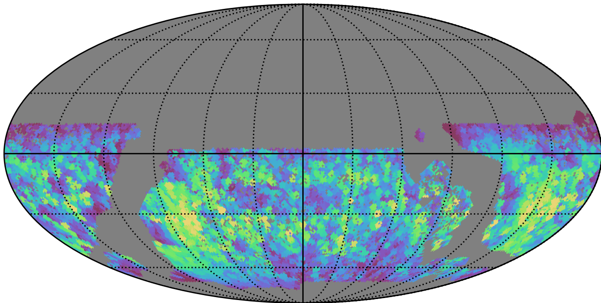
baseline_v3.0_10yrs WFD all bands: Max normairmass
