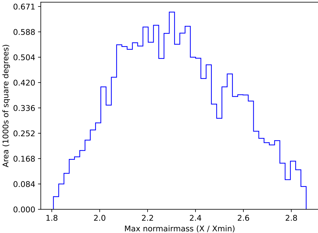
baseline_v3.0_10yrs WFD all bands: Max normairmass
