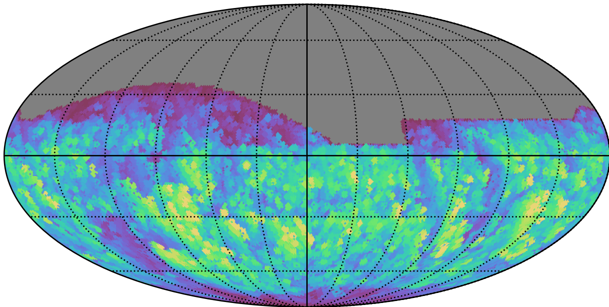
baseline_v3.0_10yrs All sky z band: Max normairmass
