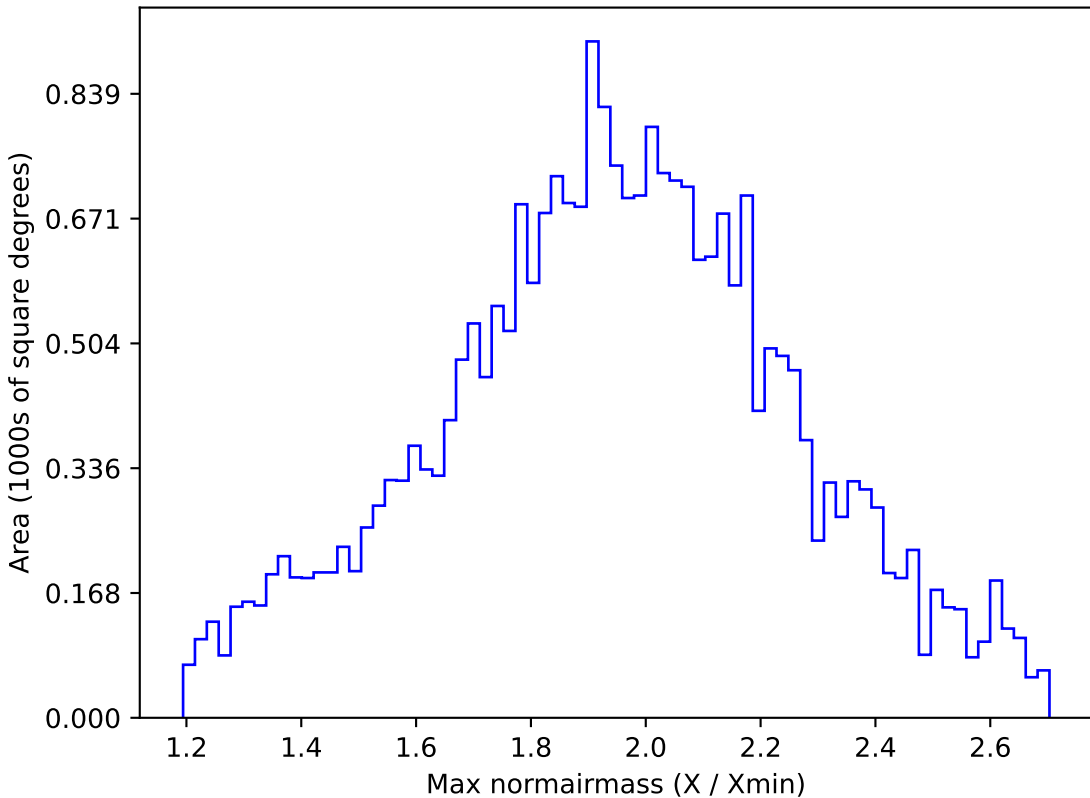
baseline_v3.0_10yrs All sky z band: Max normairmass
