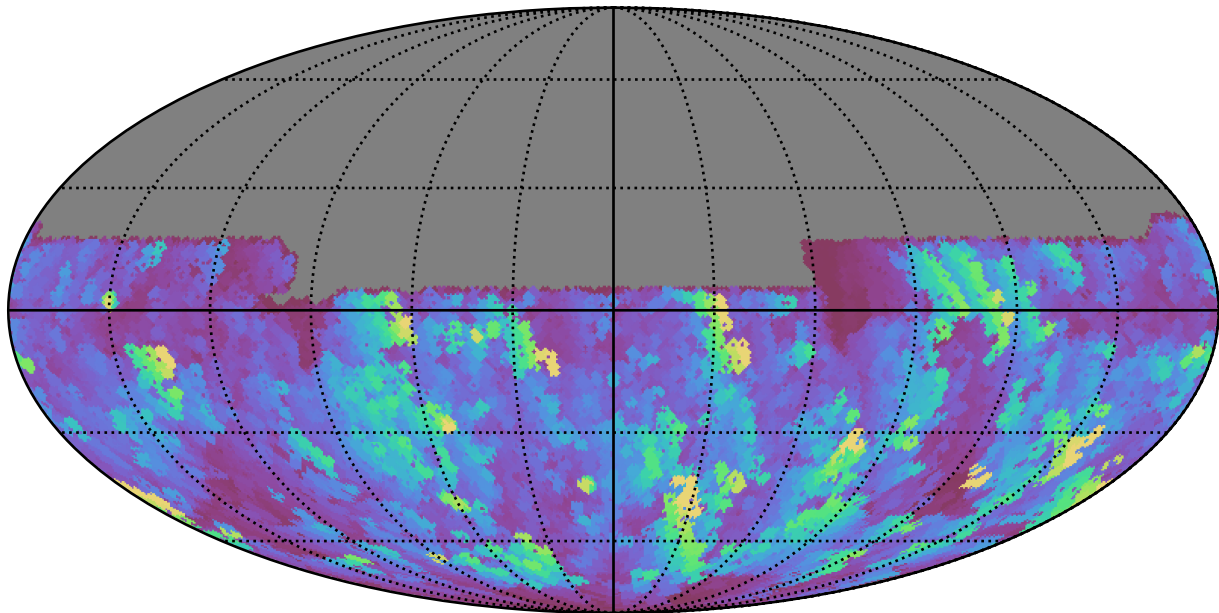
baseline_v3.0_10yrs All sky u band: Max normairmass
