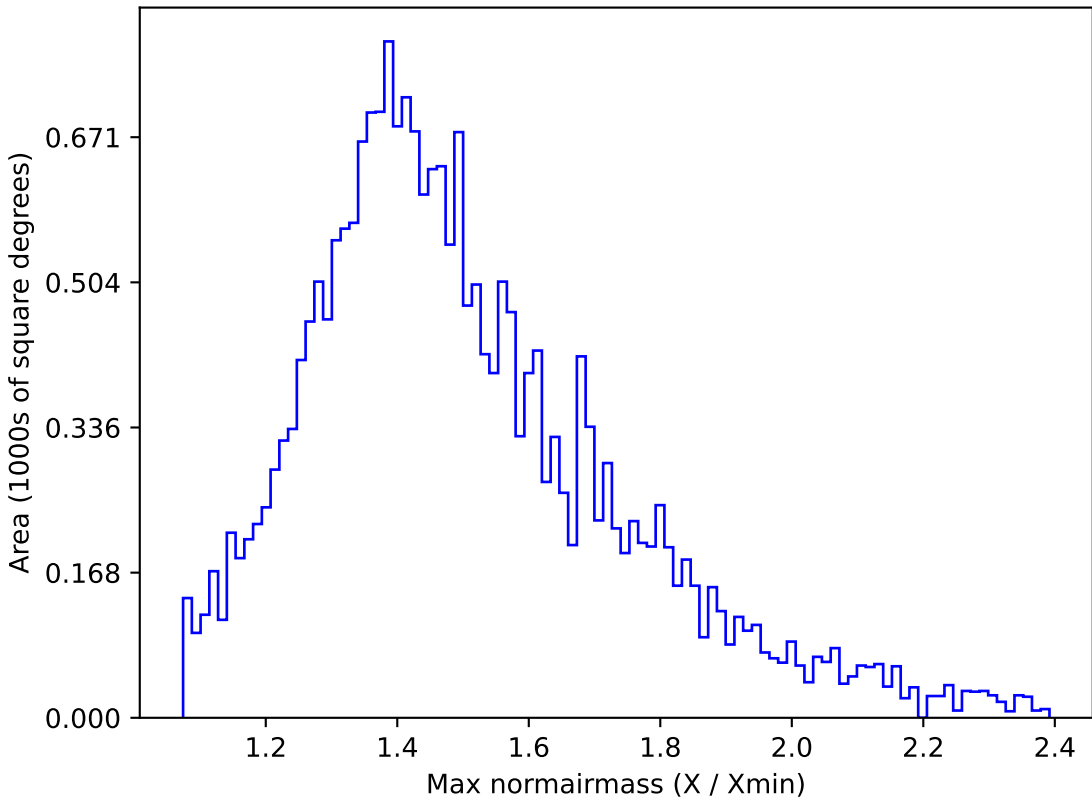
baseline_v3.0_10yrs All sky u band: Max normairmass
