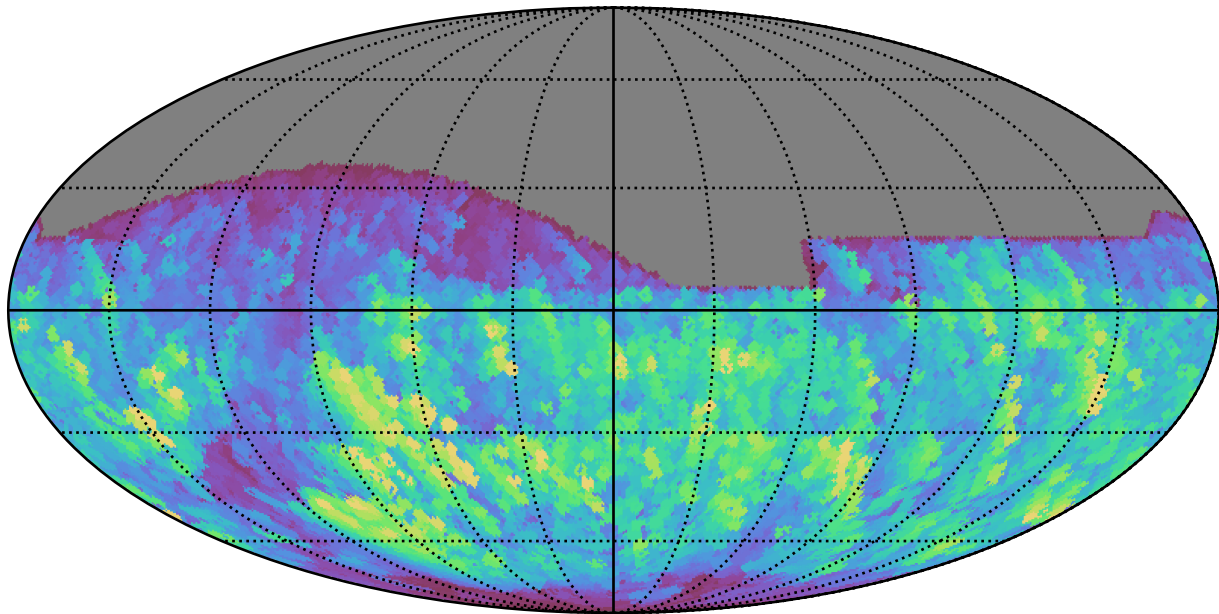
baseline_v3.0_10yrs All sky r band: Max normairmass
