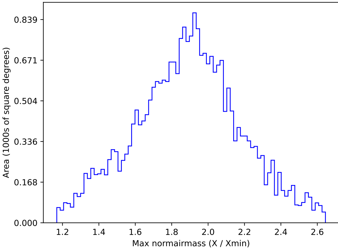
baseline_v3.0_10yrs All sky r band: Max normairmass
