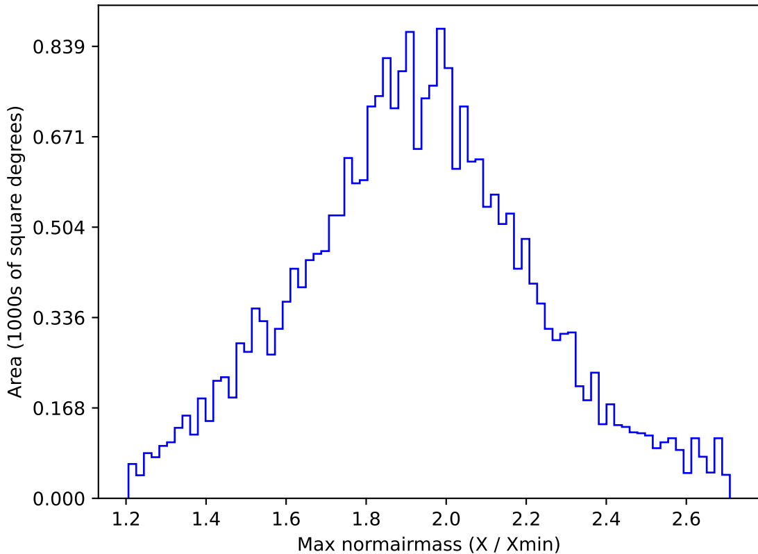
baseline_v3.0_10yrs All sky i band: Max normairmass
