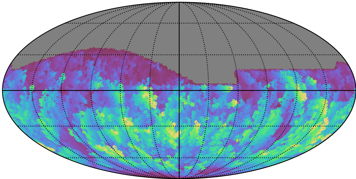
baseline_v3.0_10yrs All sky g band: Max normairmass
