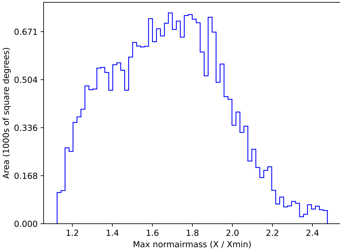
baseline_v3.0_10yrs All sky g band: Max normairmass
