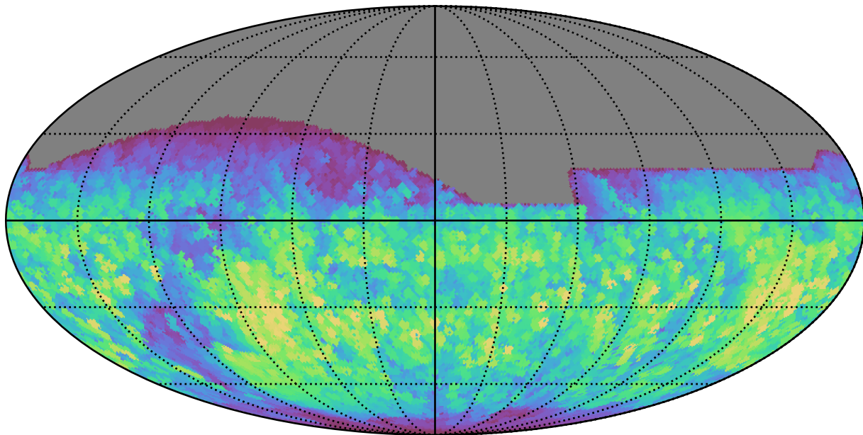
baseline_v3.0_10yrs All sky all bands: Max normairmass
