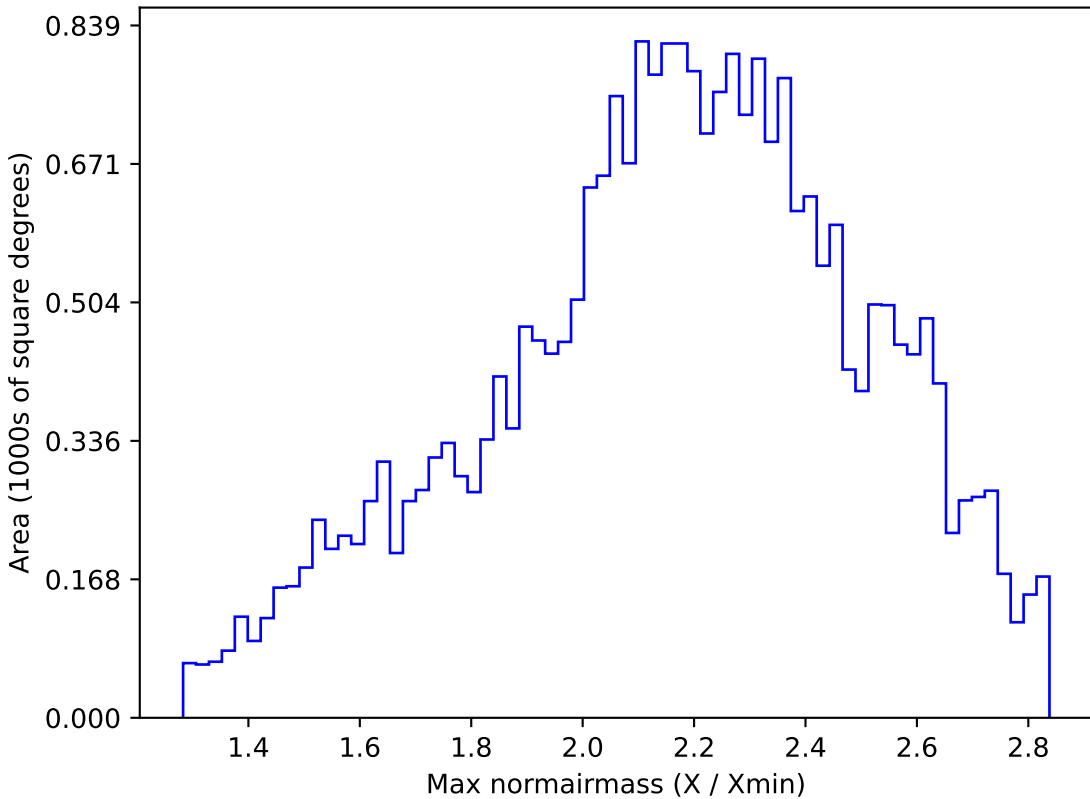
baseline_v3.0_10yrs All sky all bands: Max normairmass
