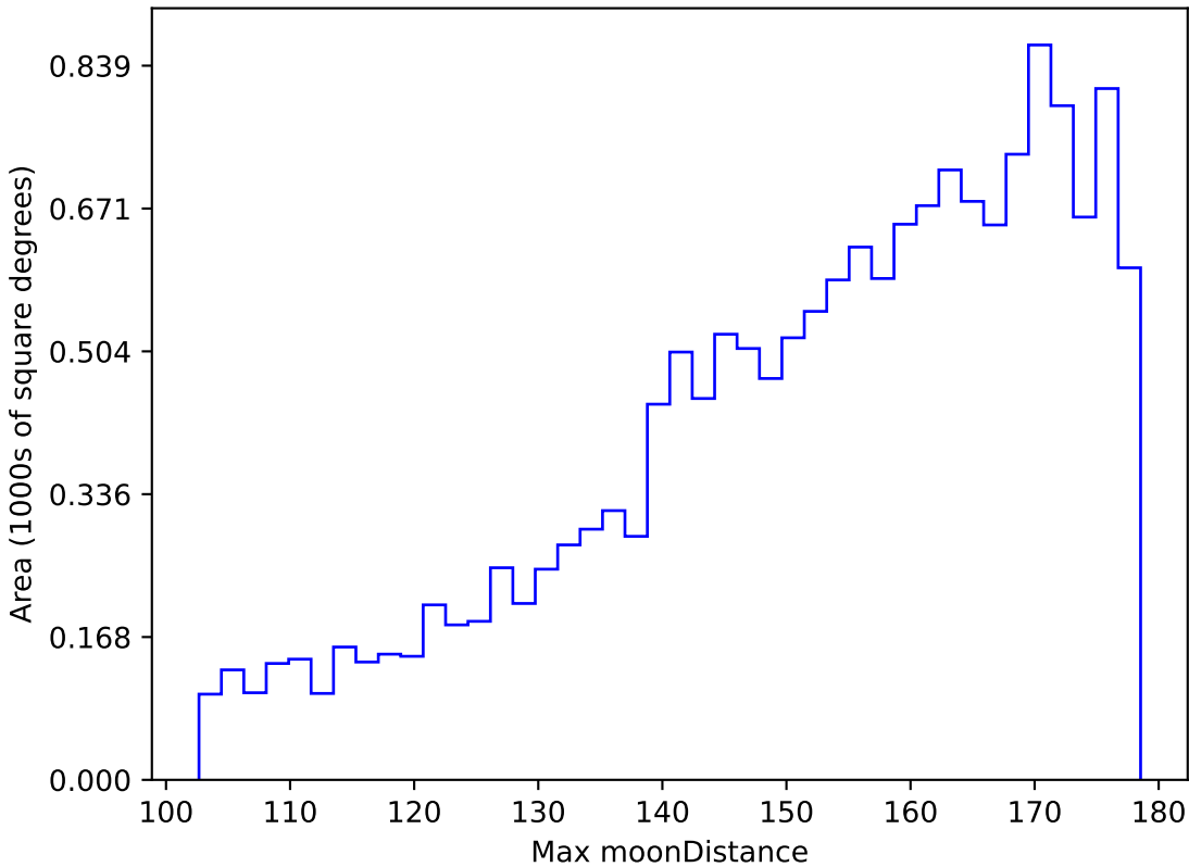
baseline_v3.0_10yrs WFD z band: Max moonDistance
