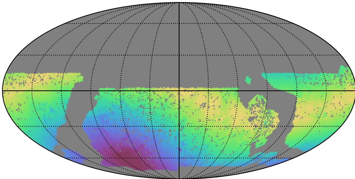
baseline_v3.0_10yrs WFD y band: Max moonDistance
