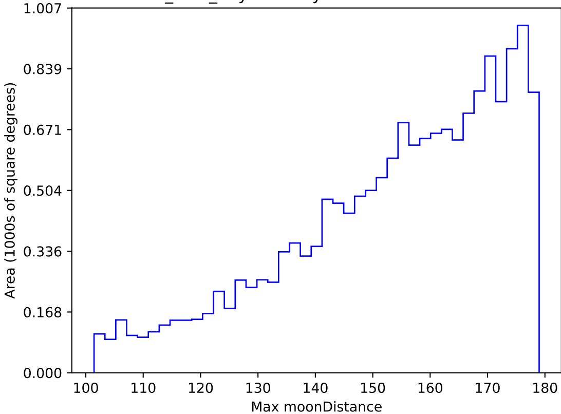
baseline_v3.0_10yrs WFD y band: Max moonDistance
