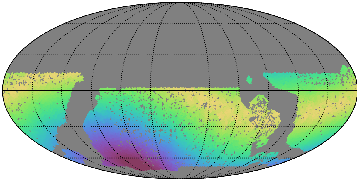
baseline_v3.0_10yrs WFD u band: Max moonDistance
