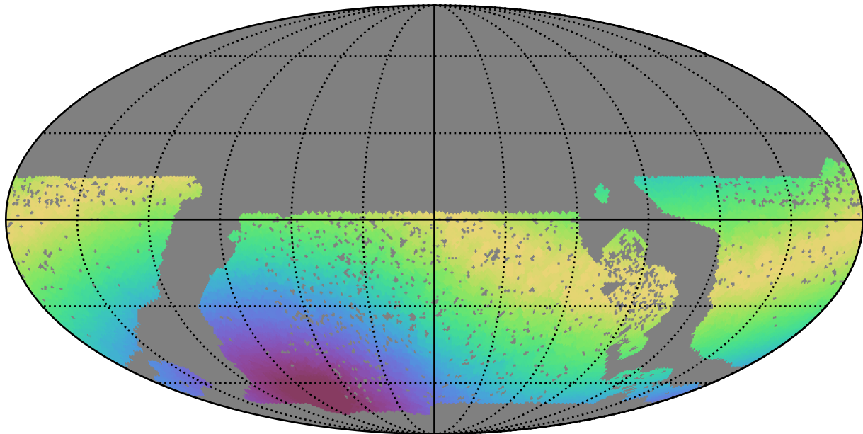
baseline_v3.0_10yrs WFD r band: Max moonDistance
