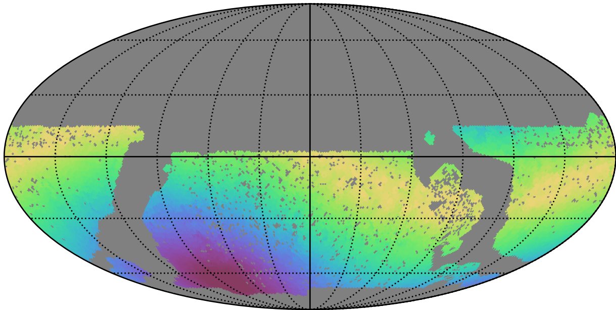
baseline_v3.0_10yrs WFD i band: Max moonDistance
