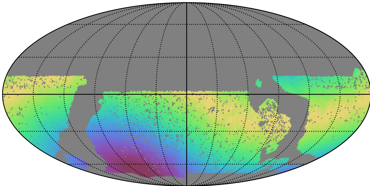
baseline_v3.0_10yrs WFD g band: Max moonDistance
