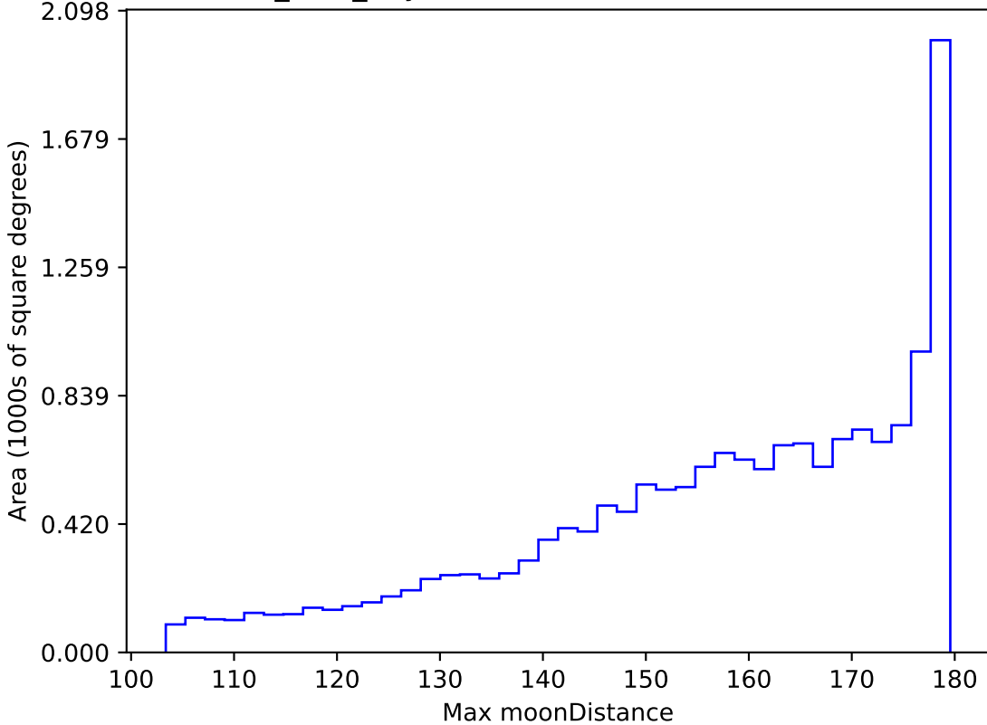
baseline_v3.0_10yrs WFD all bands: Max moonDistance
