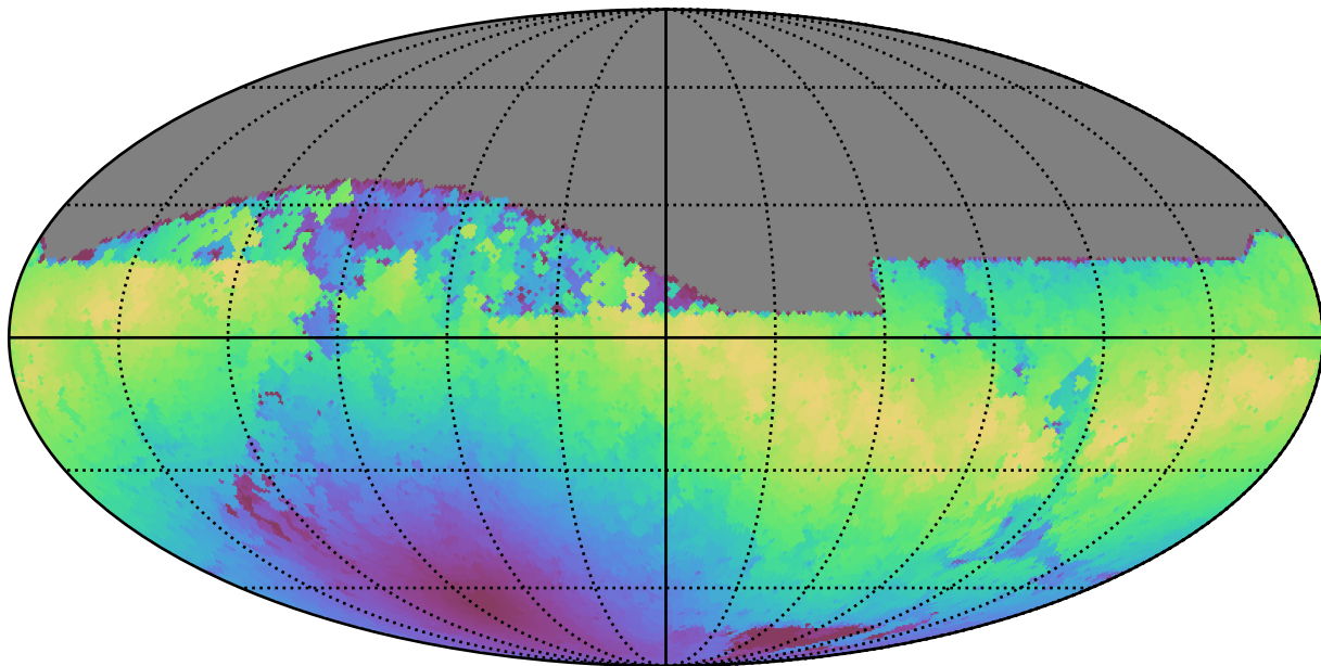
baseline_v3.0_10yrs All sky z band: Max moonDistance
