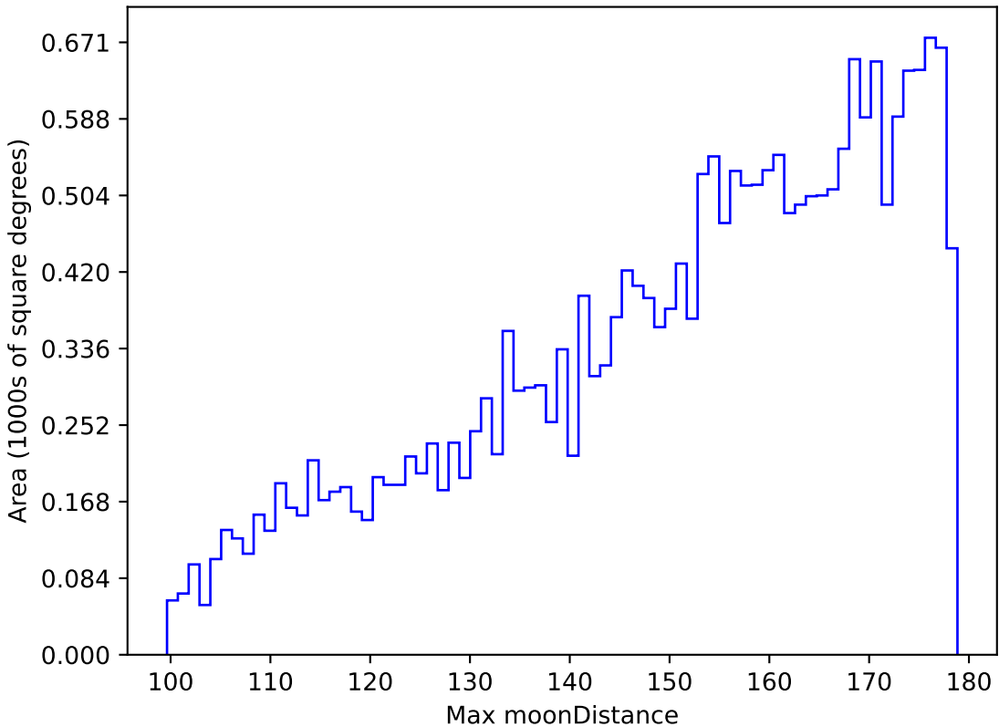
baseline_v3.0_10yrs All sky y band: Max moonDistance
