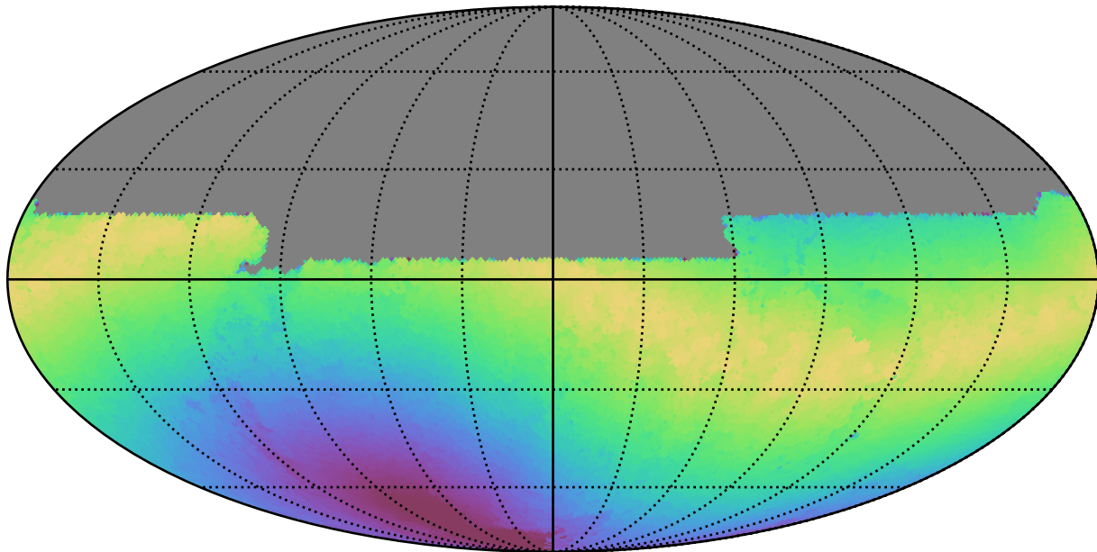
baseline_v3.0_10yrs All sky u band: Max moonDistance
