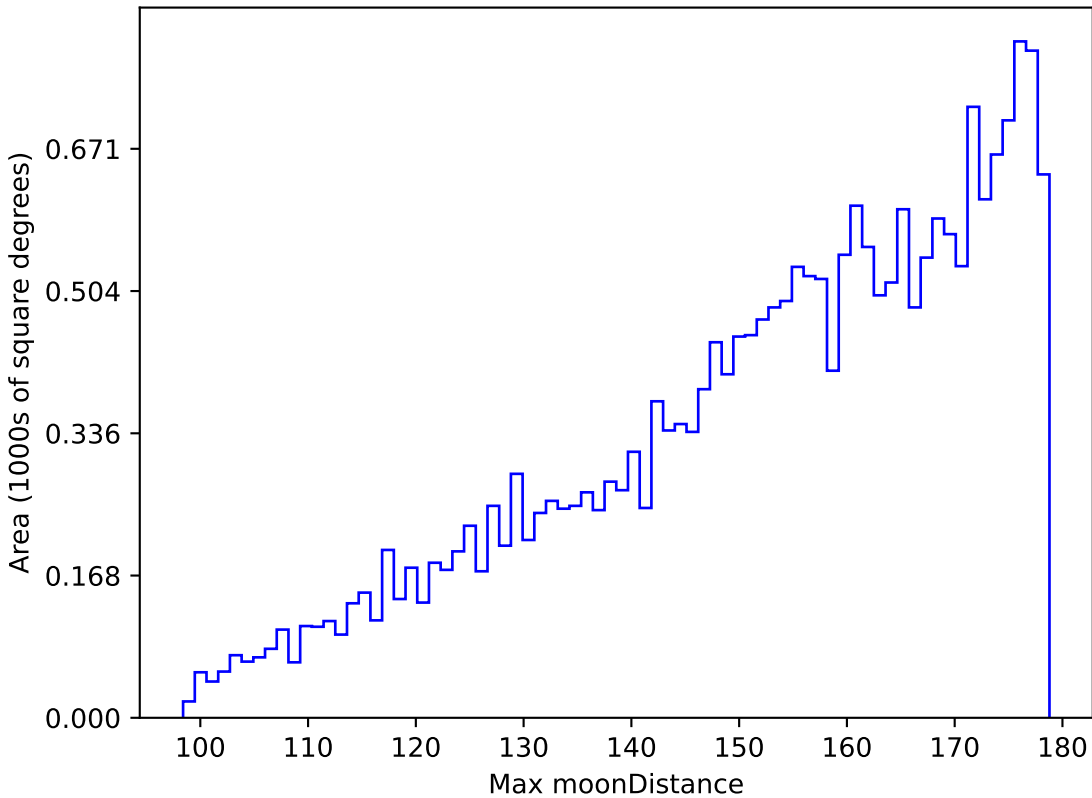
baseline_v3.0_10yrs All sky u band: Max moonDistance
