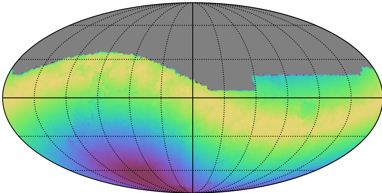
baseline_v3.0_10yrs All sky r band: Max moonDistance
