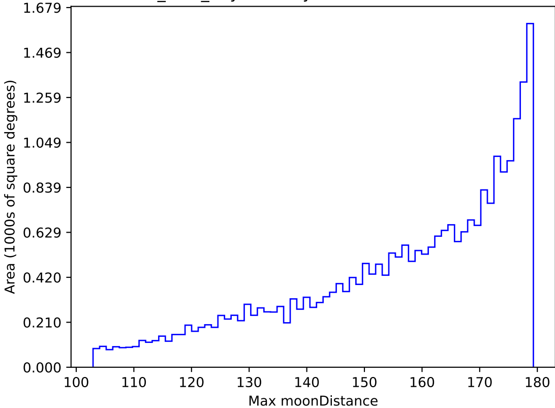
baseline_v3.0_10yrs All sky r band: Max moonDistance
