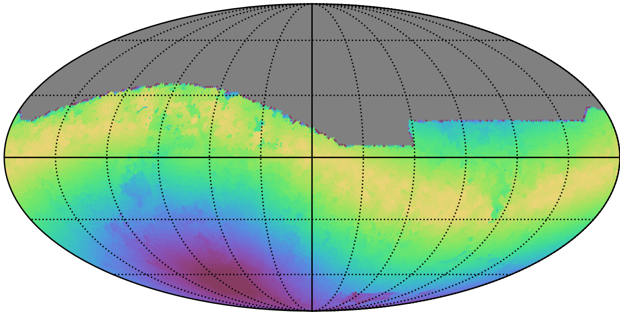
baseline_v3.0_10yrs All sky i band: Max moonDistance
