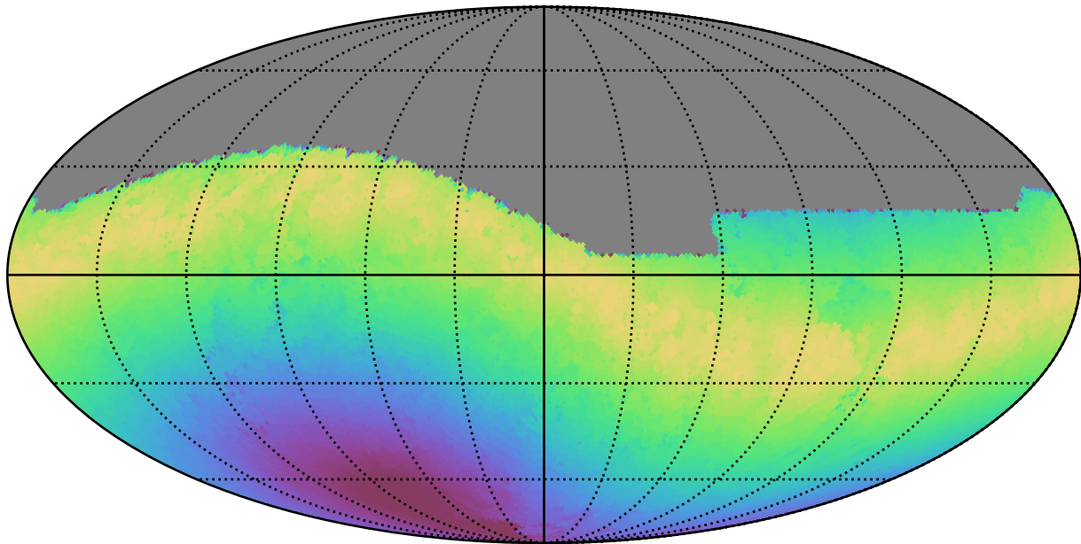
baseline_v3.0_10yrs All sky g band: Max moonDistance
