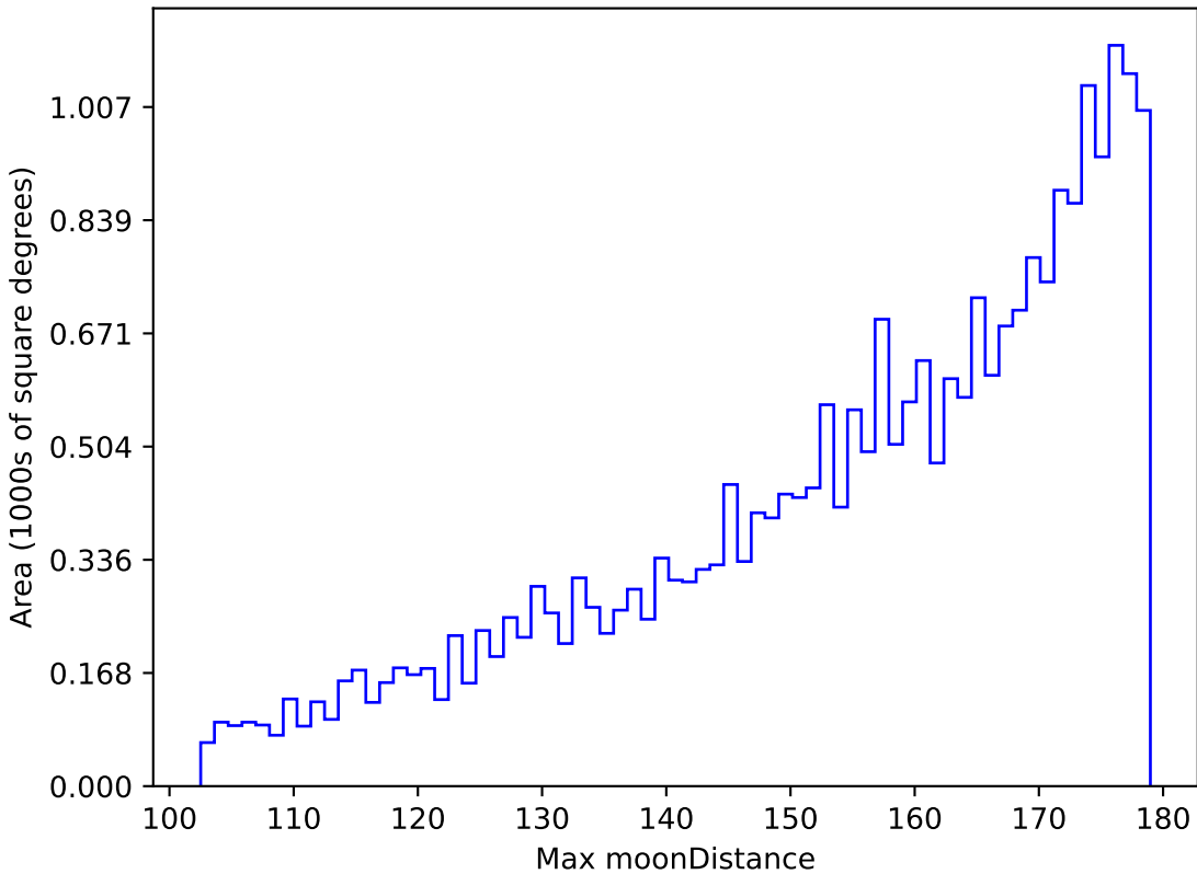
baseline_v3.0_10yrs All sky g band: Max moonDistance
