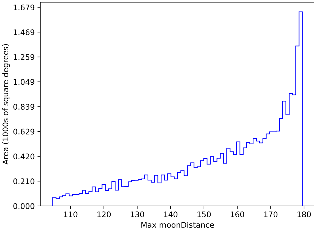
baseline_v3.0_10yrs All sky all bands: Max moonDistance
