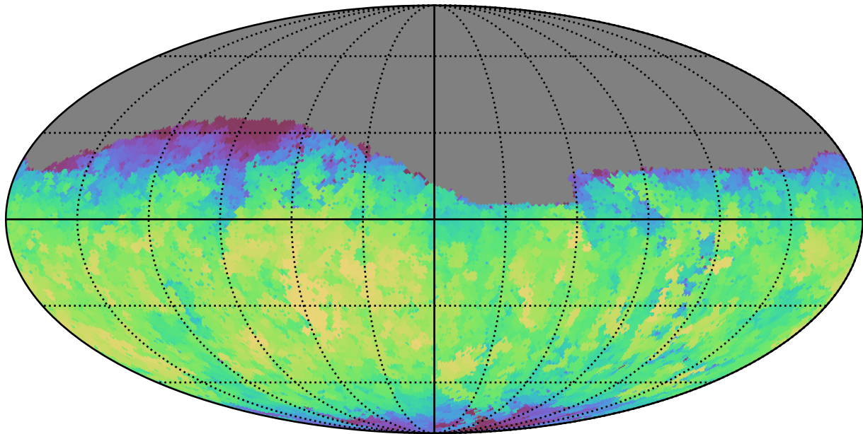
baseline_v3.0_10yrs Yr 1 z band: Max fiveSigmaDepth
