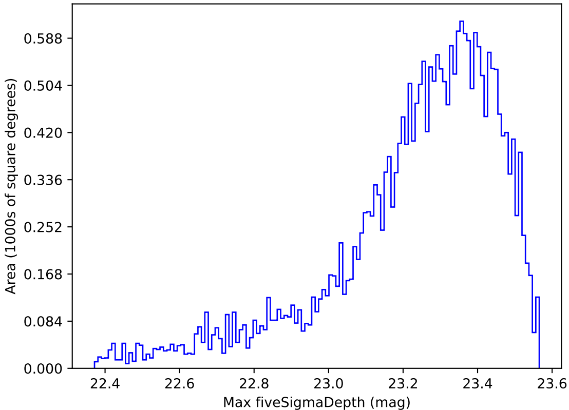
baseline_v3.0_10yrs Yr 1 z band: Max fiveSigmaDepth
