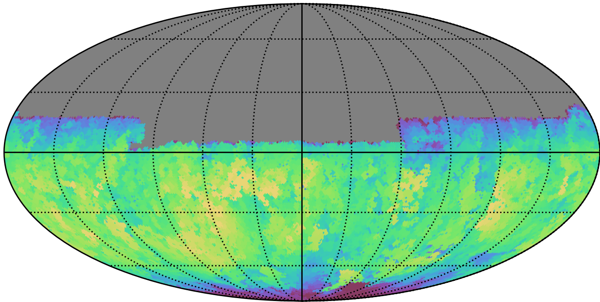
baseline_v3.0_10yrs Yr 1 y band: Max fiveSigmaDepth
