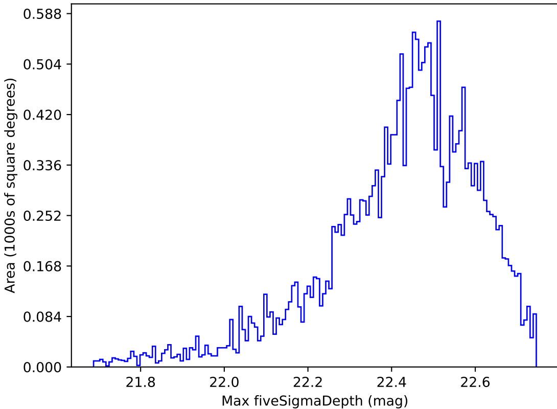
baseline_v3.0_10yrs Yr 1 y band: Max fiveSigmaDepth
