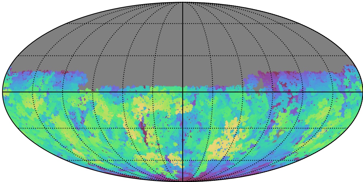
baseline_v3.0_10yrs Yr 1 u band: Max fiveSigmaDepth
