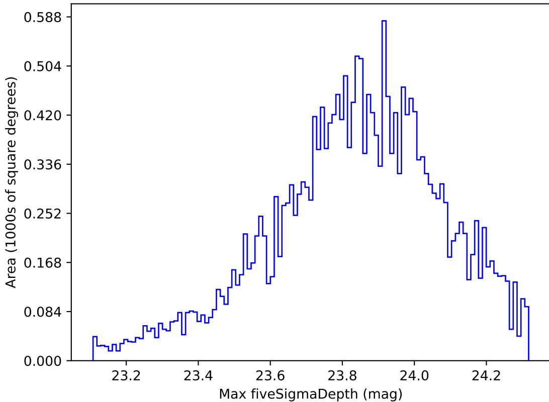
baseline_v3.0_10yrs Yr 1 u band: Max fiveSigmaDepth
