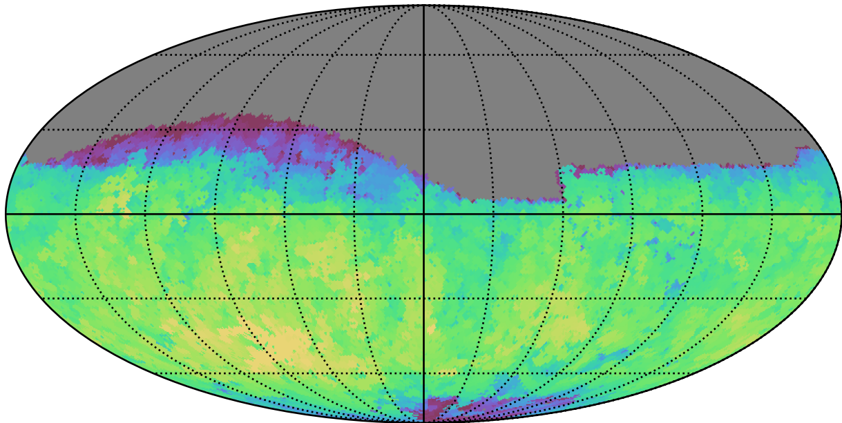
baseline_v3.0_10yrs Yr 1 r band: Max fiveSigmaDepth
