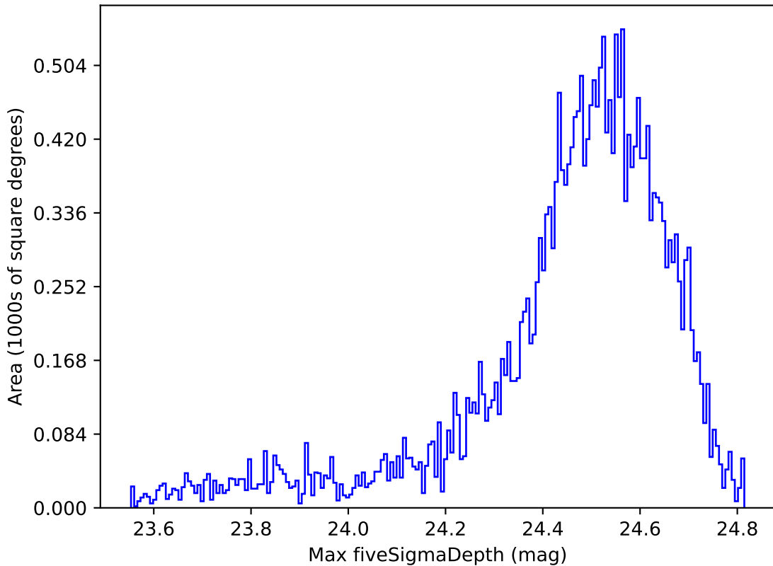
baseline_v3.0_10yrs Yr 1 r band: Max fiveSigmaDepth
