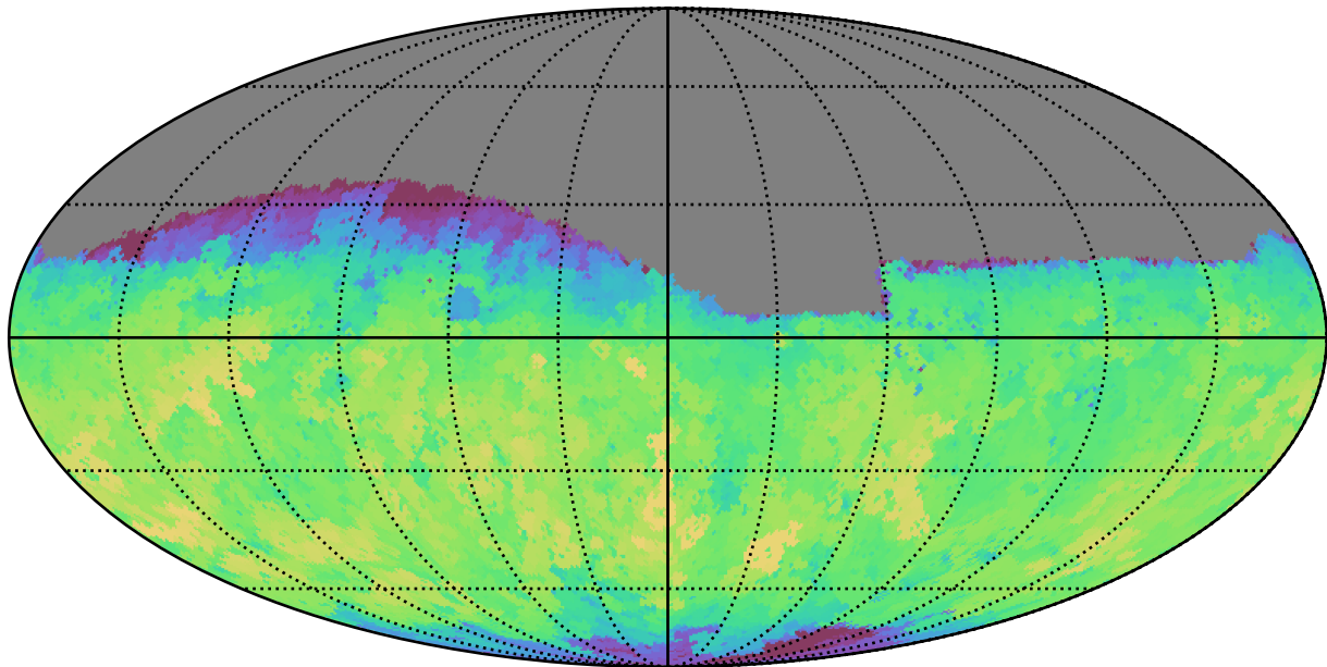
baseline_v3.0_10yrs Yr 1 i band: Max fiveSigmaDepth
