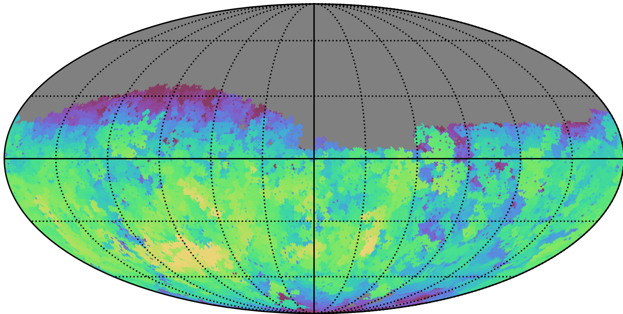
baseline_v3.0_10yrs Yr 1 g band: Max fiveSigmaDepth
