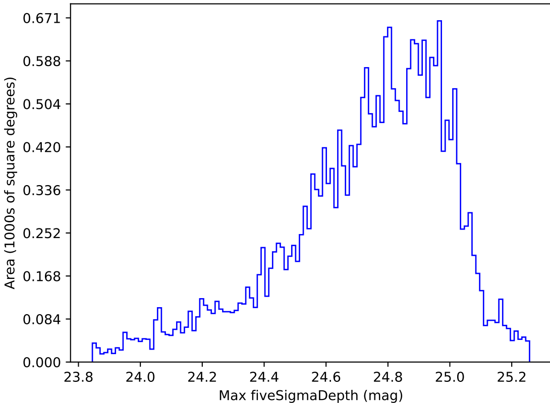
baseline_v3.0_10yrs Yr 1 g band: Max fiveSigmaDepth
