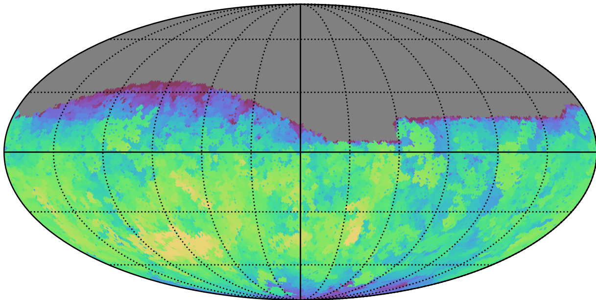
baseline_v3.0_10yrs Yr 1 all bands: Max fiveSigmaDepth
